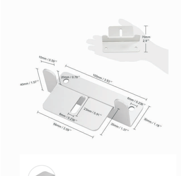
Long Shape Hole for Universal Use
